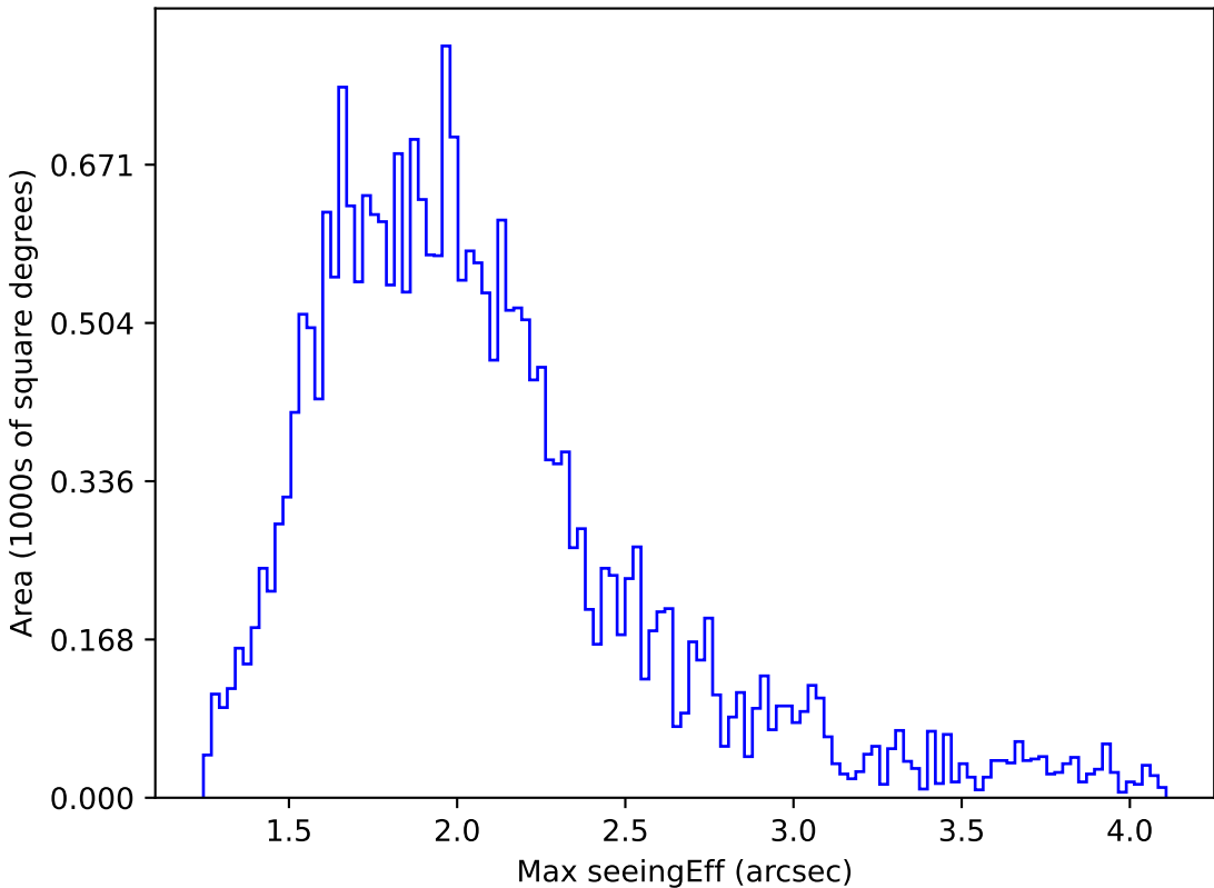
too_elab_r16_d2_griz_v3.4_10yrs Yr 1 all bands: Max seeingEff
