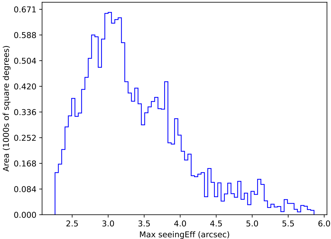
too_elab_r16_d2_griz_v3.4_10yrs WFD all bands: Max seeingEff
