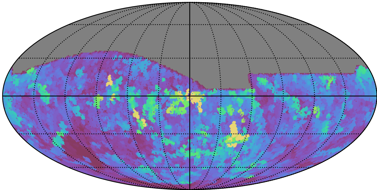
too_elab_r16_d2_griz_v3.4_10yrs All sky z band: Max seeingEff
