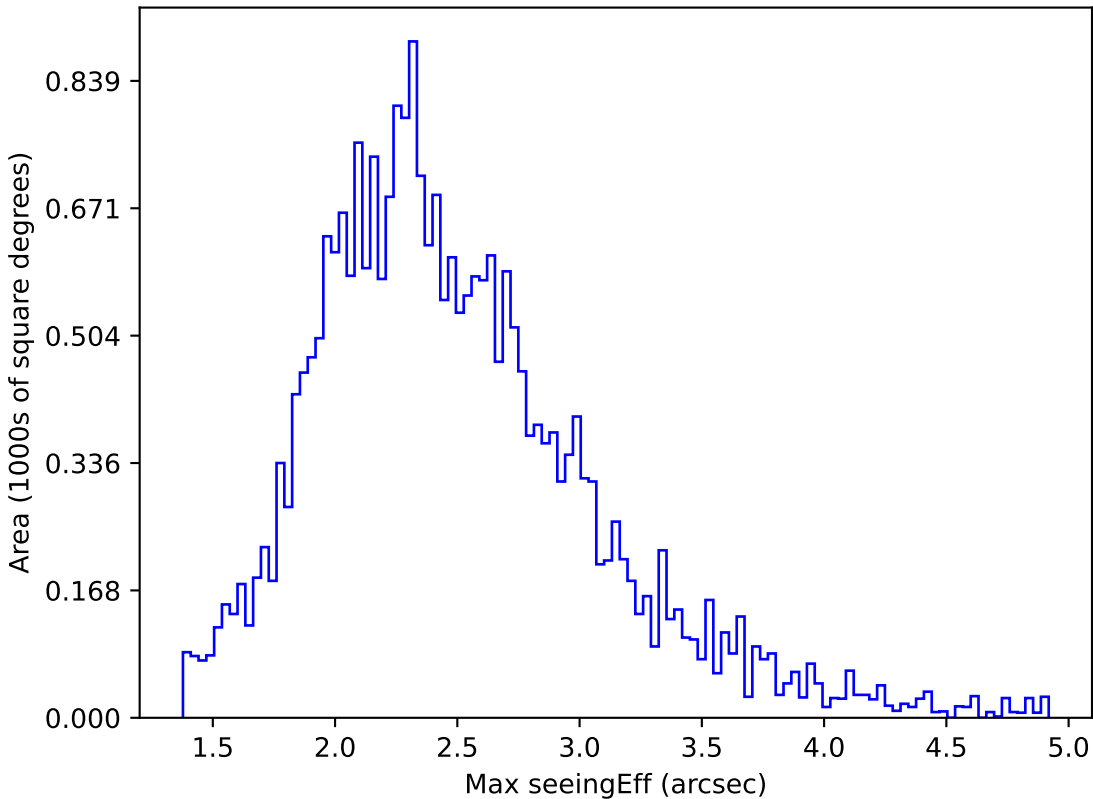
too_elab_r16_d2_griz_v3.4_10yrs All sky z band: Max seeingEff
