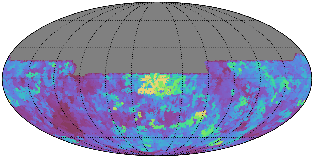
too_elab_r16_d2_griz_v3.4_10yrs All sky y band: Max seeingEff
