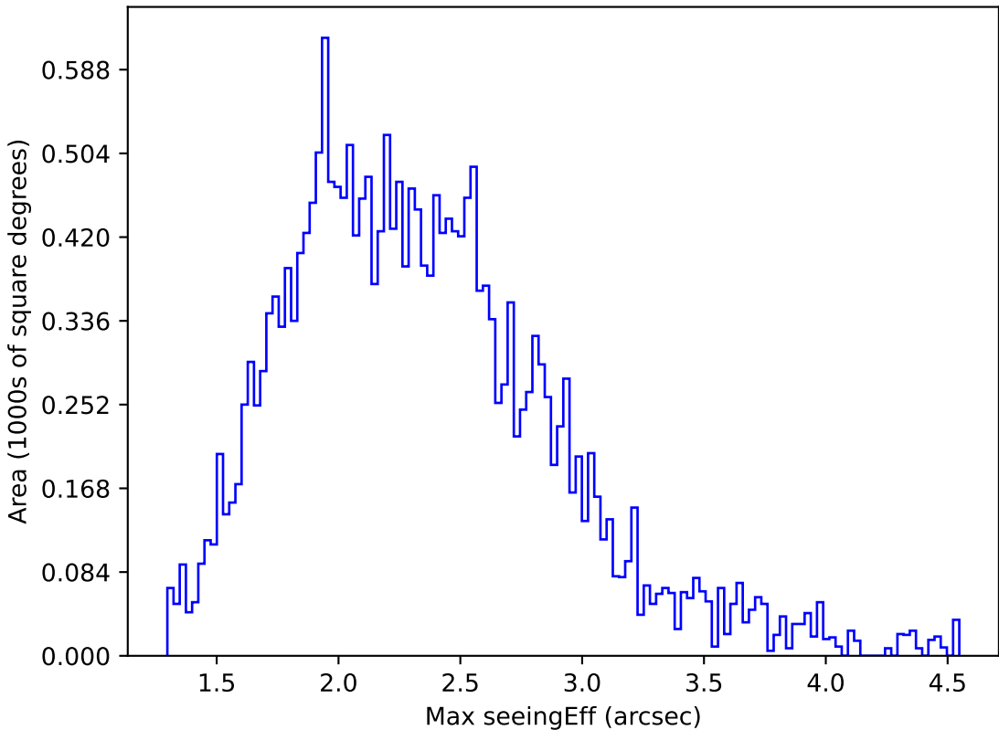
too_elab_r16_d2_griz_v3.4_10yrs All sky y band: Max seeingEff
