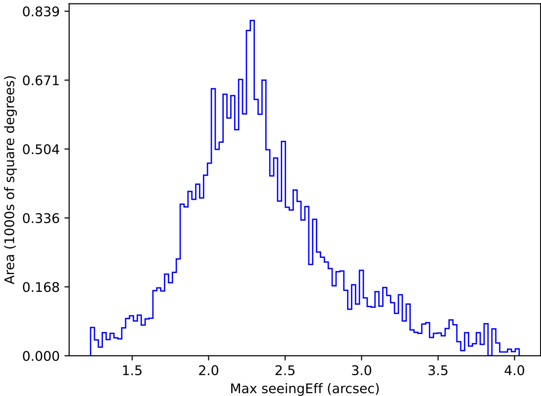
too_elab_r16_d2_griz_v3.4_10yrs All sky u band: Max seeingEff
