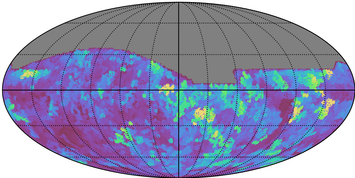
too_elab_r16_d2_griz_v3.4_10yrs All sky r band: Max seeingEff
