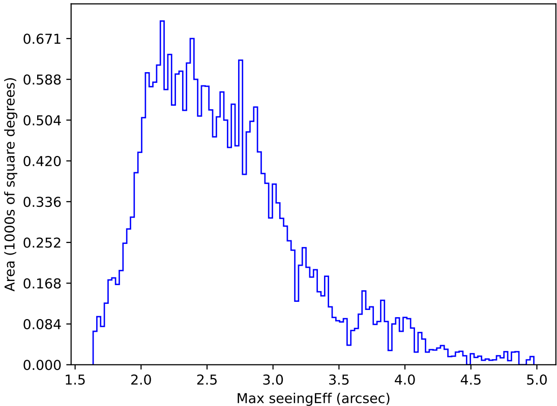
too_elab_r16_d2_griz_v3.4_10yrs All sky r band: Max seeingEff
