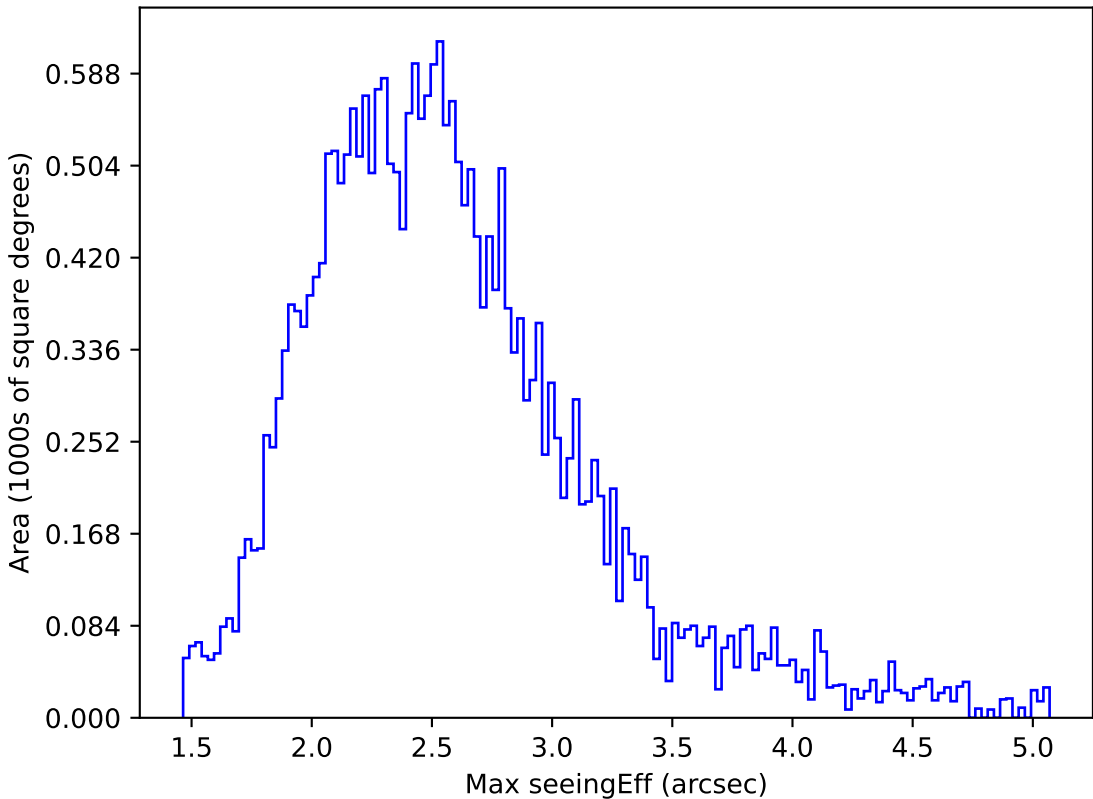
too_elab_r16_d2_griz_v3.4_10yrs All sky i band: Max seeingEff
