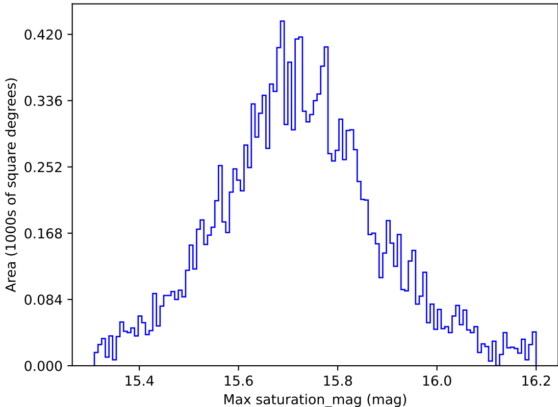
too_elab_r16_d2_griz_v3.4_10yrs WFD g band: Max saturation_mag
