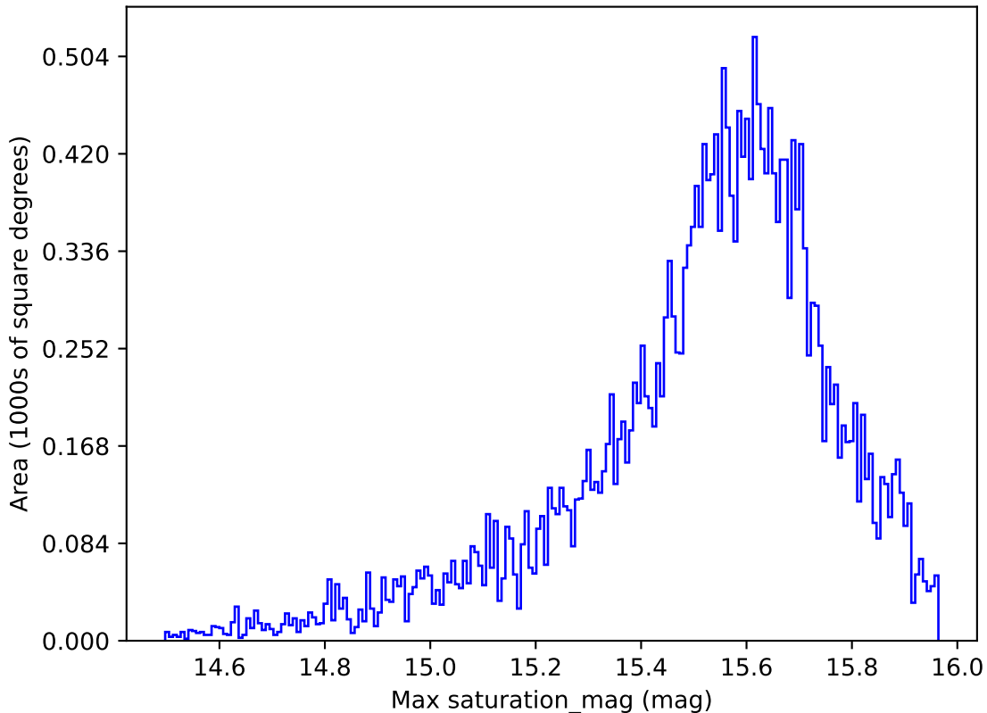
too_elab_r16_d2_griz_v3.4_10yrs All sky i band: Max saturation_mag
