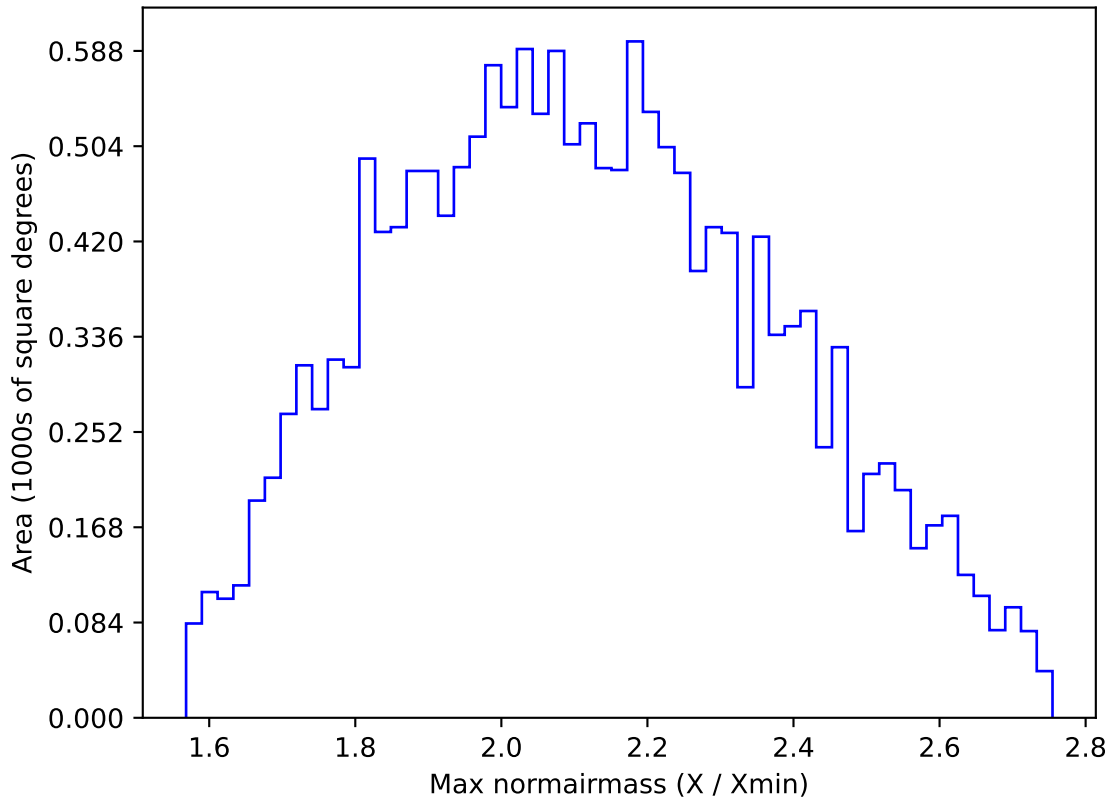
too_elab_r16_d2_griz_v3.4_10yrs WFD y band: Max normairmass
