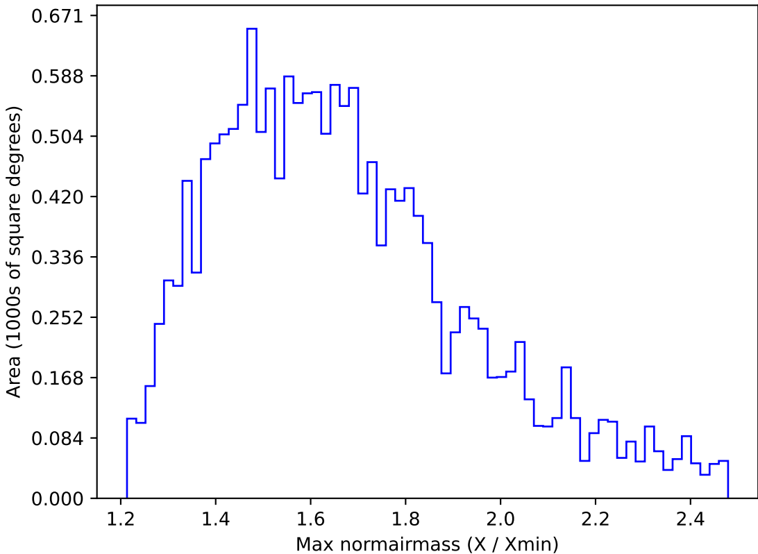
too_elab_r16_d2_griz_v3.4_10yrs WFD u band: Max normairmass
