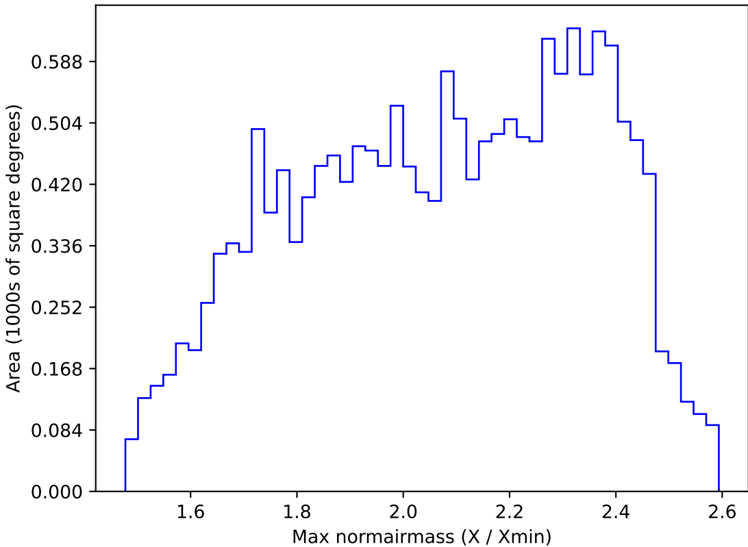
too_elab_r16_d2_griz_v3.4_10yrs WFD r band: Max normairmass
