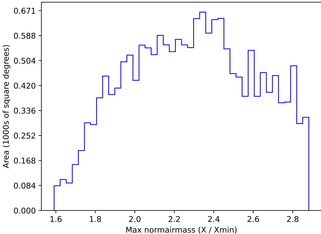
too_elab_r16_d2_griz_v3.4_10yrs WFD i band: Max normairmass
