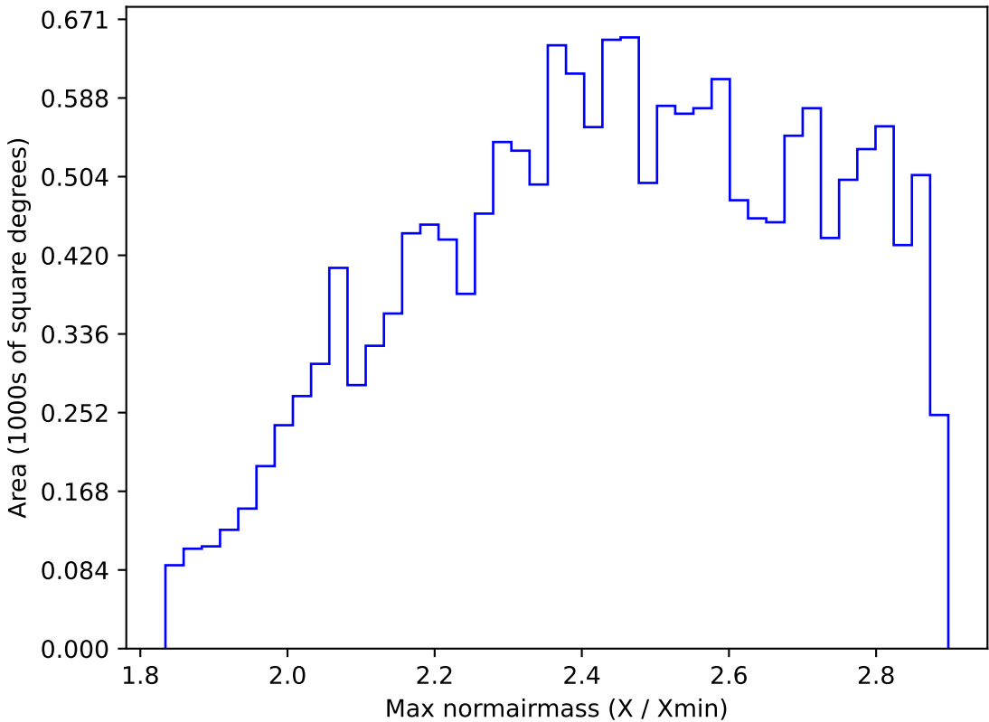
too_elab_r16_d2_griz_v3.4_10yrs WFD all bands: Max normairmass
