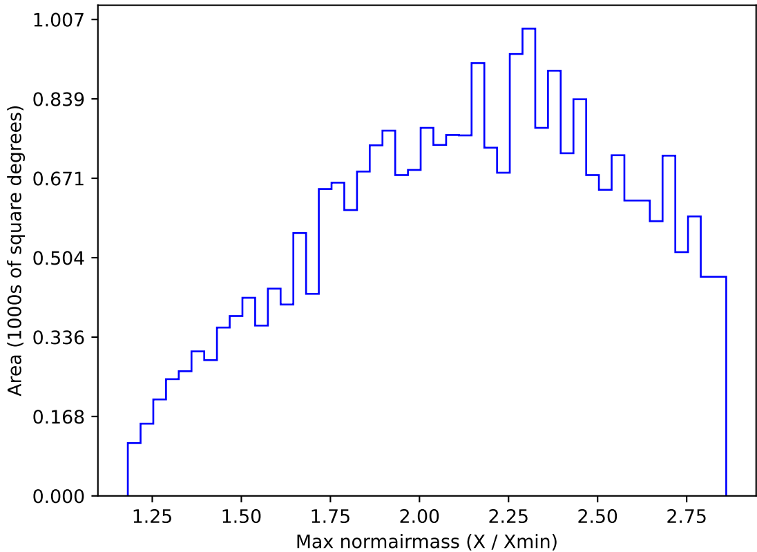
too_elab_r16_d2_griz_v3.4_10yrs All sky z band: Max normairmass
