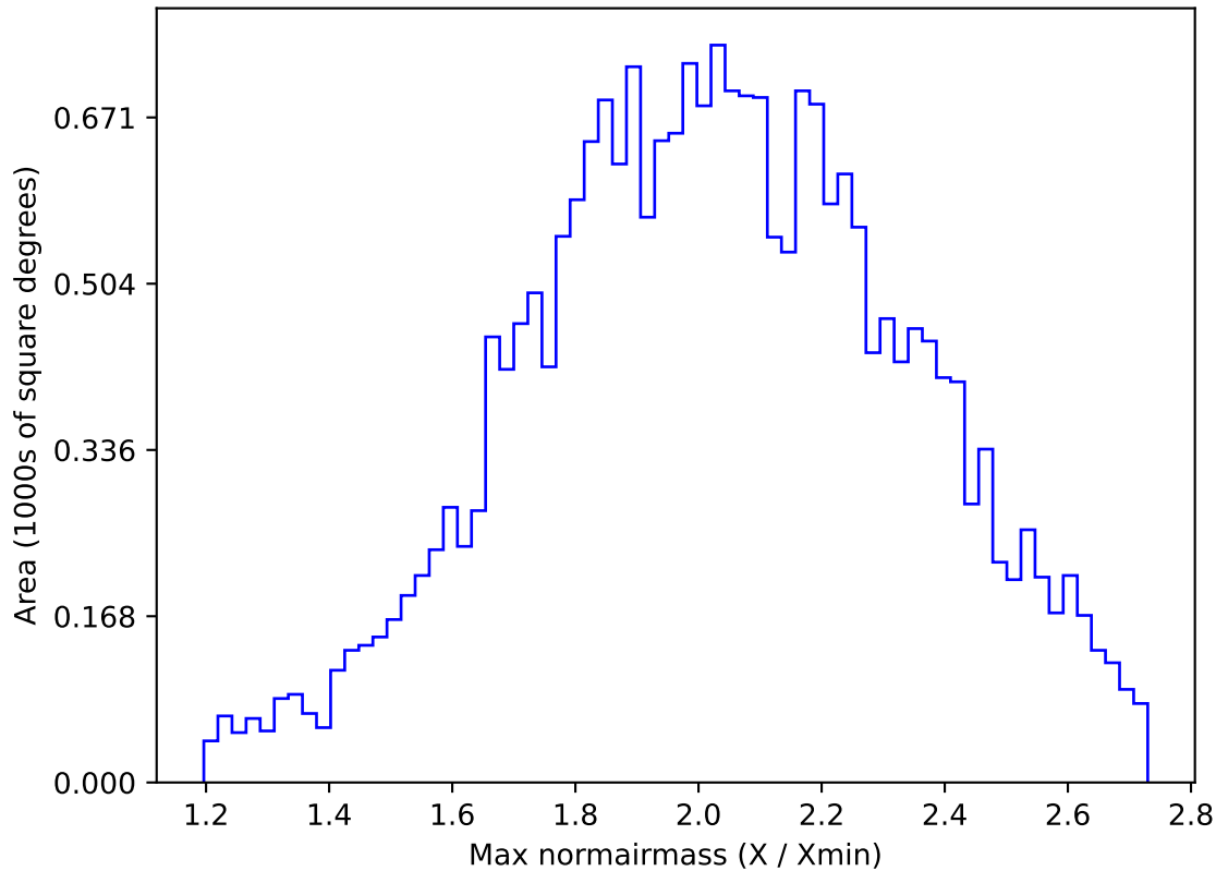
too_elab_r16_d2_griz_v3.4_10yrs All sky y band: Max normairmass
