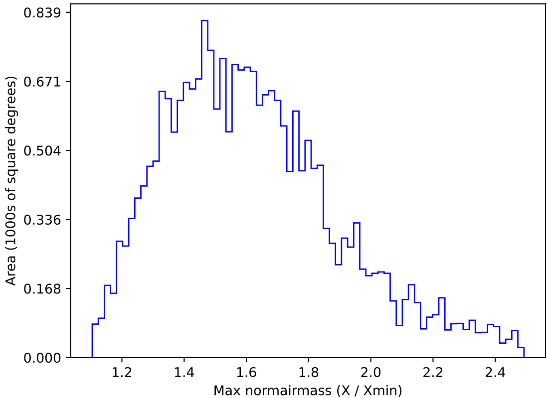
too_elab_r16_d2_griz_v3.4_10yrs All sky u band: Max normairmass
