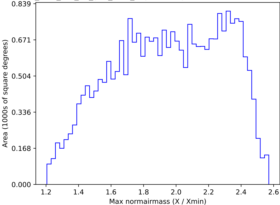
too_elab_r16_d2_griz_v3.4_10yrs All sky r band: Max normairmass
