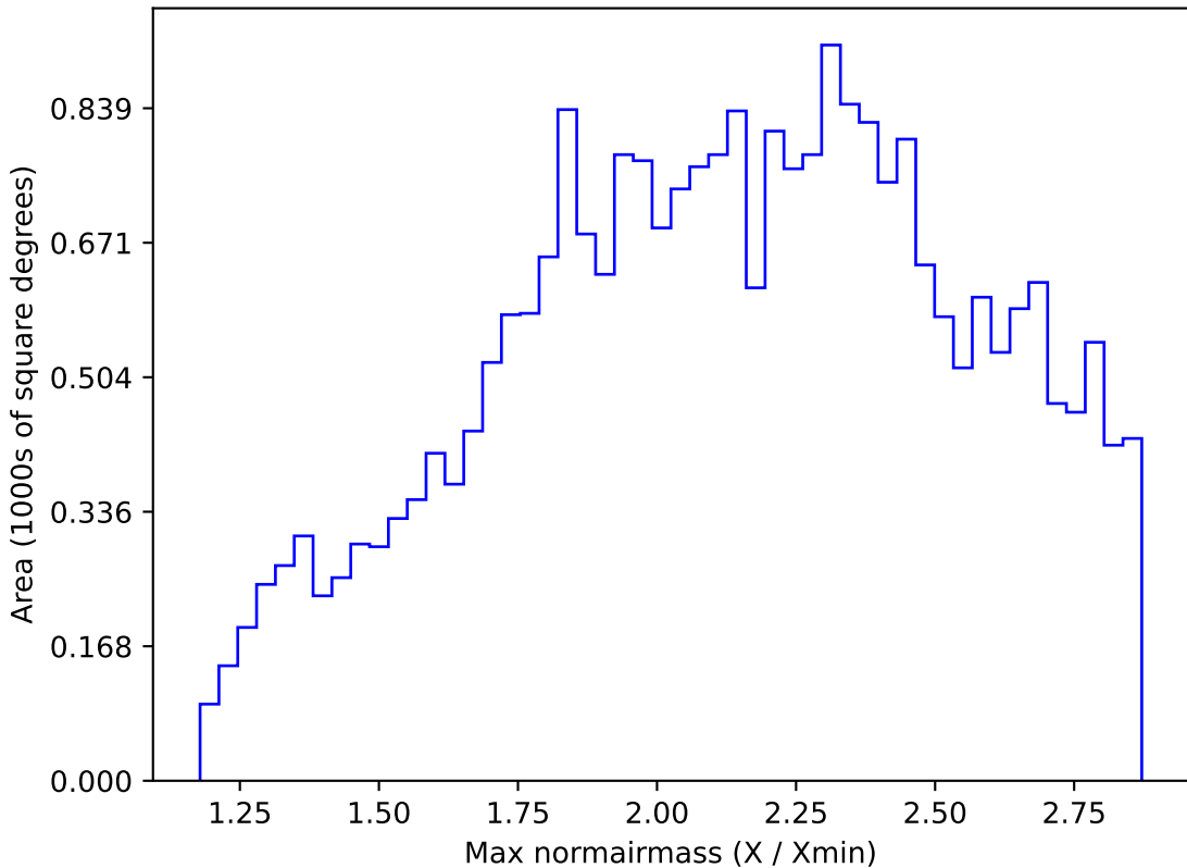
too_elab_r16_d2_griz_v3.4_10yrs All sky i band: Max normairmass
