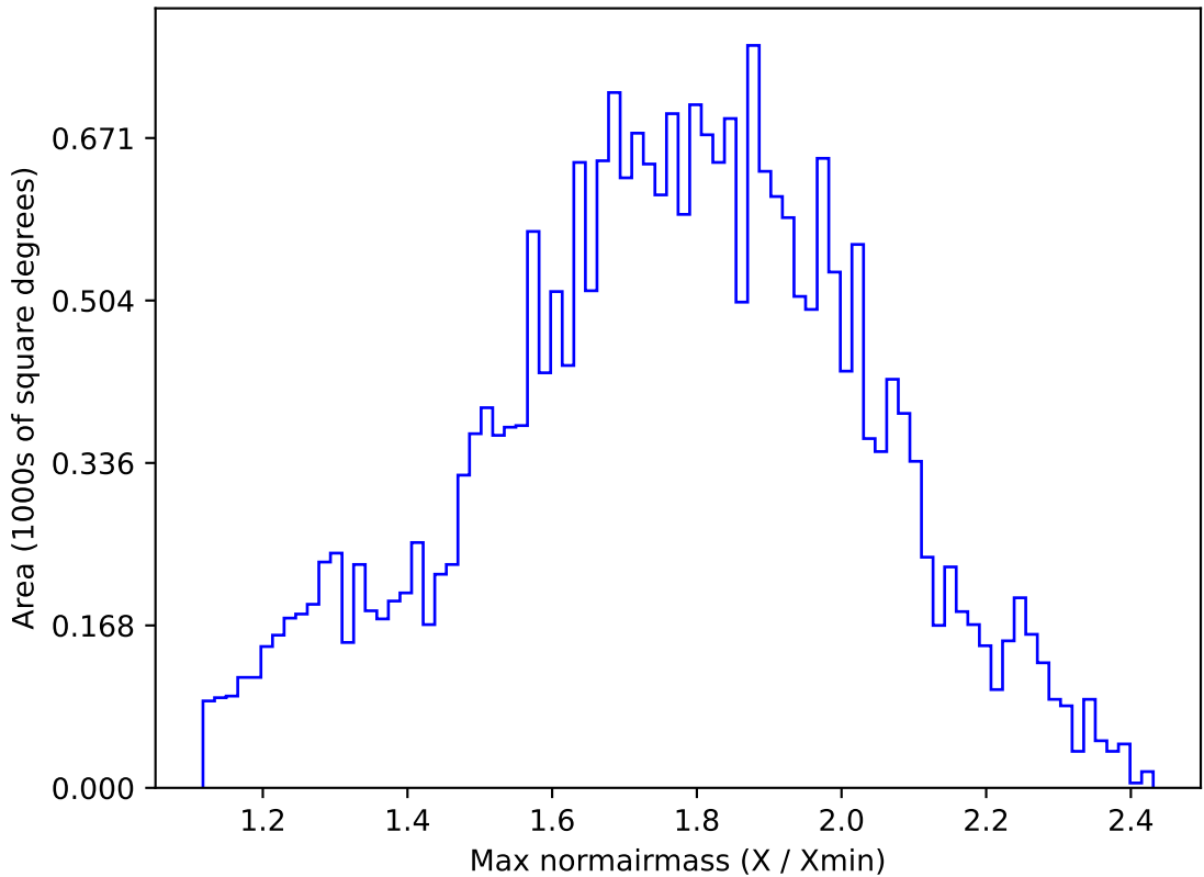
too_elab_r16_d2_griz_v3.4_10yrs All sky g band: Max normairmass
