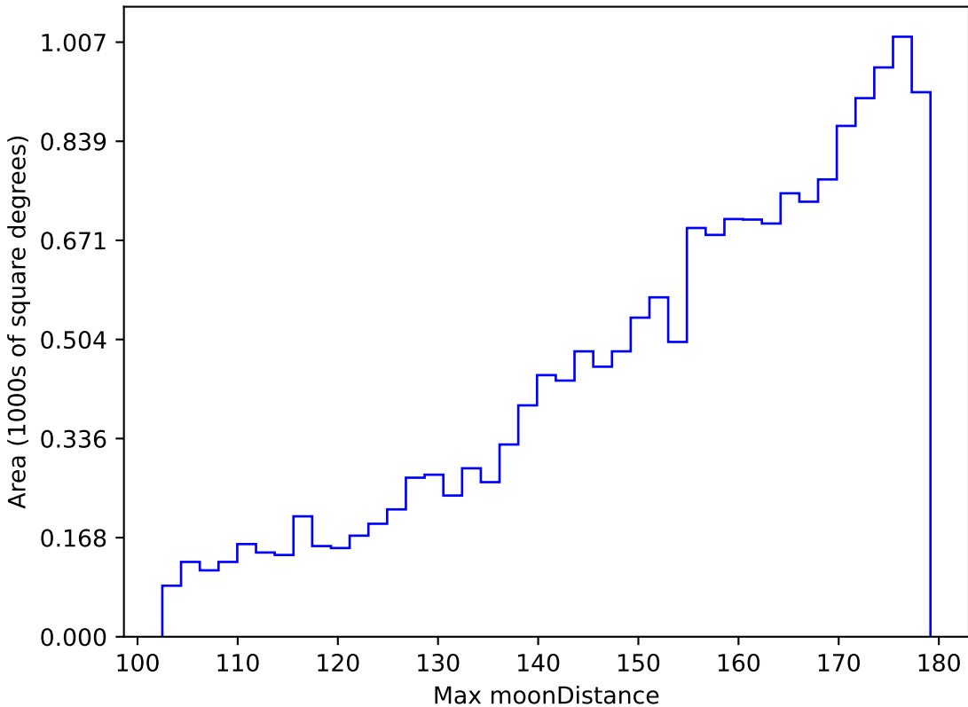
too_elab_r16_d2_griz_v3.4_10yrs WFD z band: Max moonDistance
