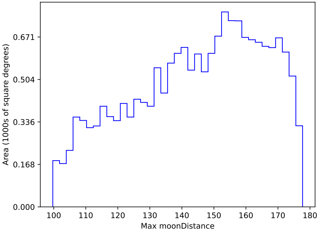
too_elab_r16_d2_griz_v3.4_10yrs WFD y band: Max moonDistance
