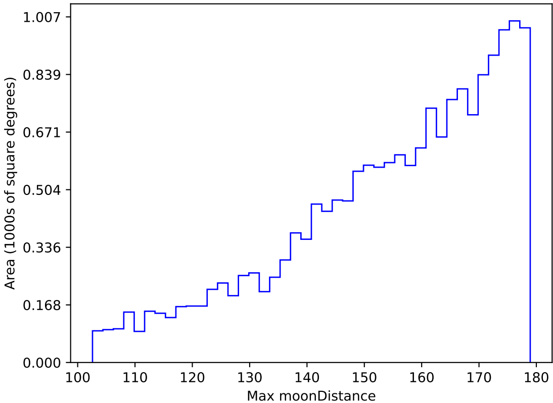
too_elab_r16_d2_griz_v3.4_10yrs WFD u band: Max moonDistance
