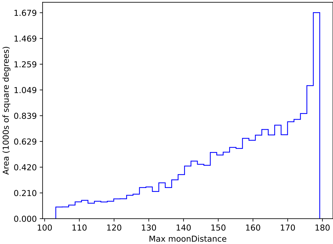
too_elab_r16_d2_griz_v3.4_10yrs WFD r band: Max moonDistance
