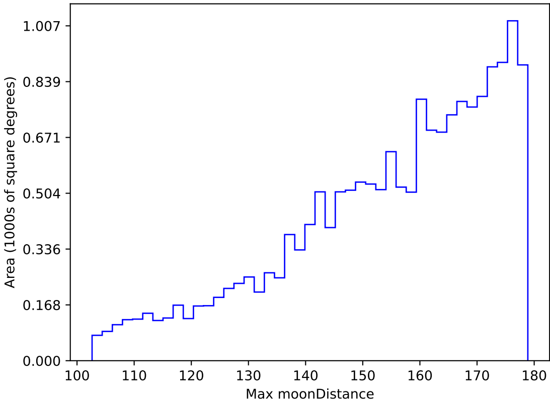
too_elab_r16_d2_griz_v3.4_10yrs WFD g band: Max moonDistance
