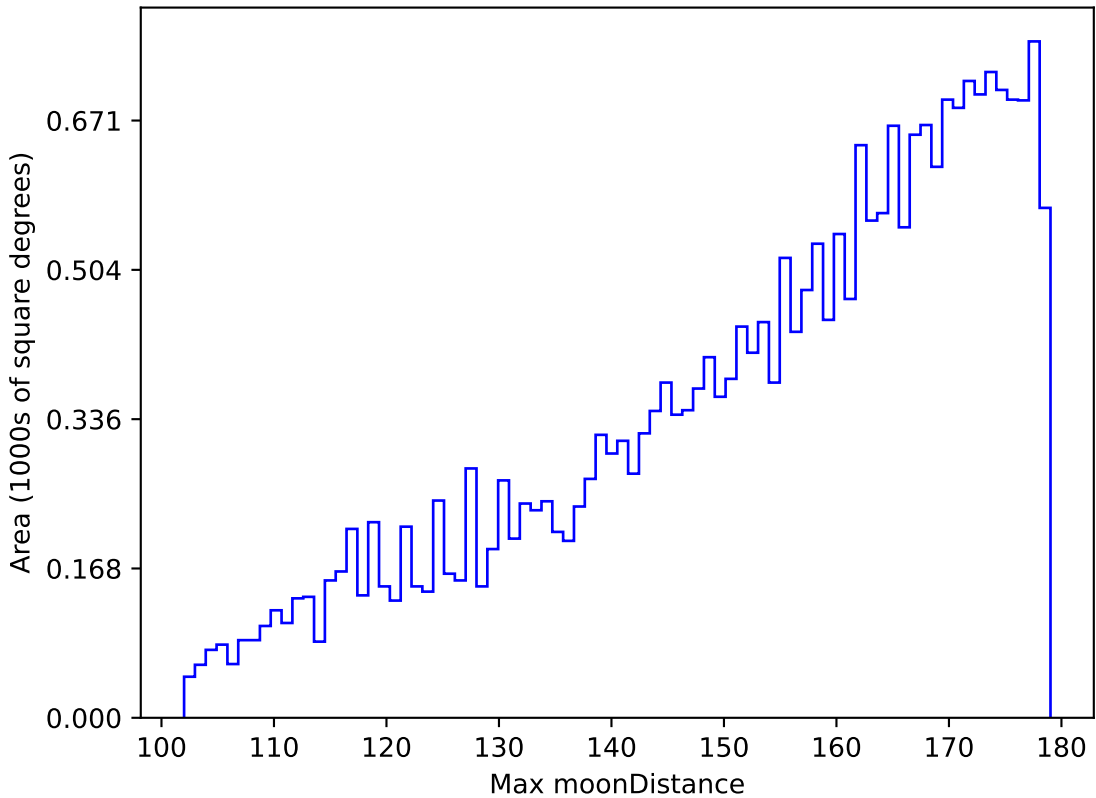
too_elab_r16_d2_griz_v3.4_10yrs All sky z band: Max moonDistance
