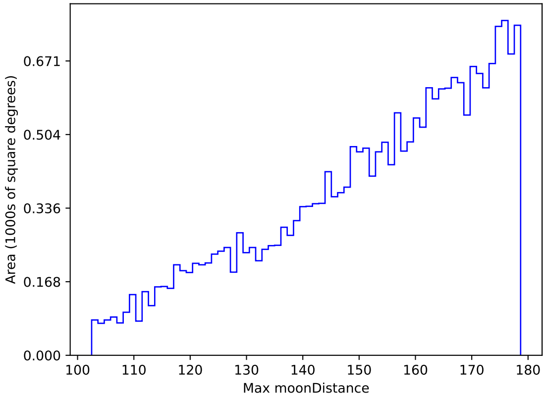
too_elab_r16_d2_griz_v3.4_10yrs All sky u band: Max moonDistance
