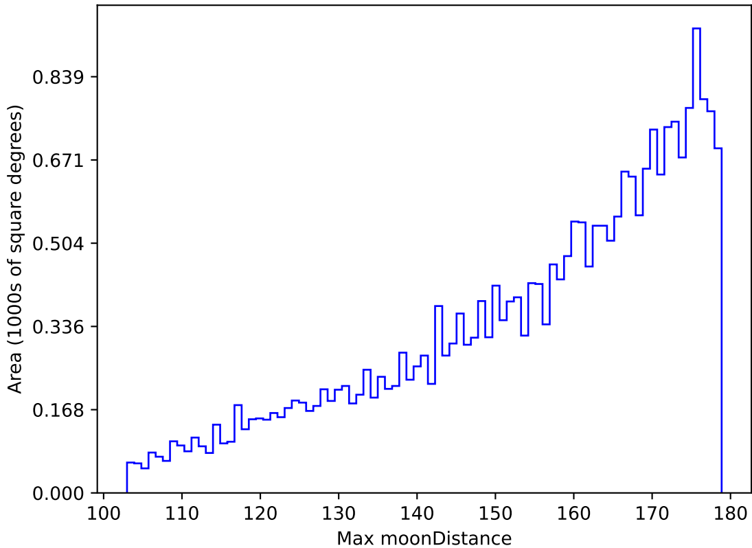
too_elab_r16_d2_griz_v3.4_10yrs All sky g band: Max moonDistance
