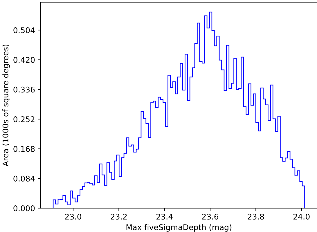
too_elab_r16_d2_griz_v3.4_10yrs Yr 1 u band: Max fiveSigmaDepth
