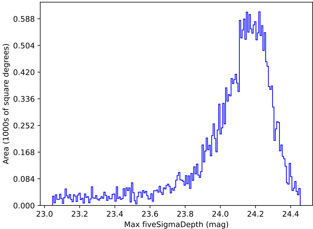
too_elab_r16_d2_griz_v3.4_10yrs Yr 1 i band: Max fiveSigmaDepth
