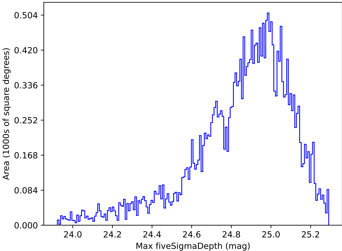
too_elab_r16_d2_griz_v3.4_10yrs Yr 1 g band: Max fiveSigmaDepth
