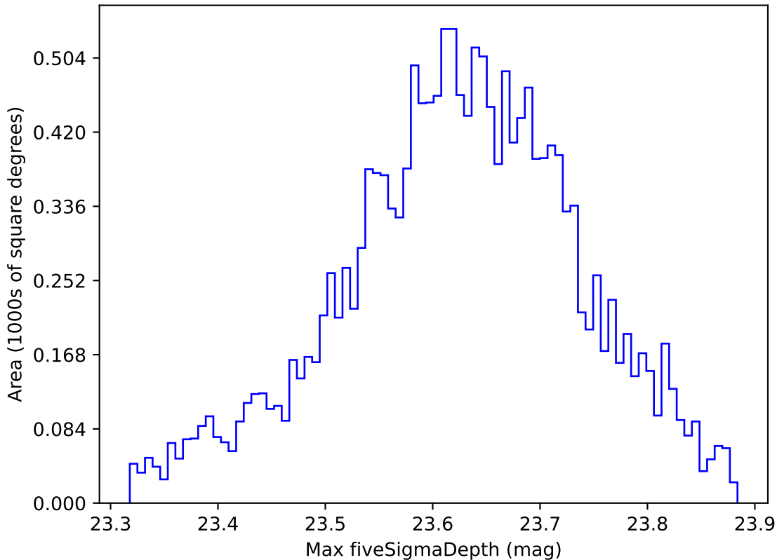
too_elab_r16_d2_griz_v3.4_10yrs WFD z band: Max fiveSigmaDepth
