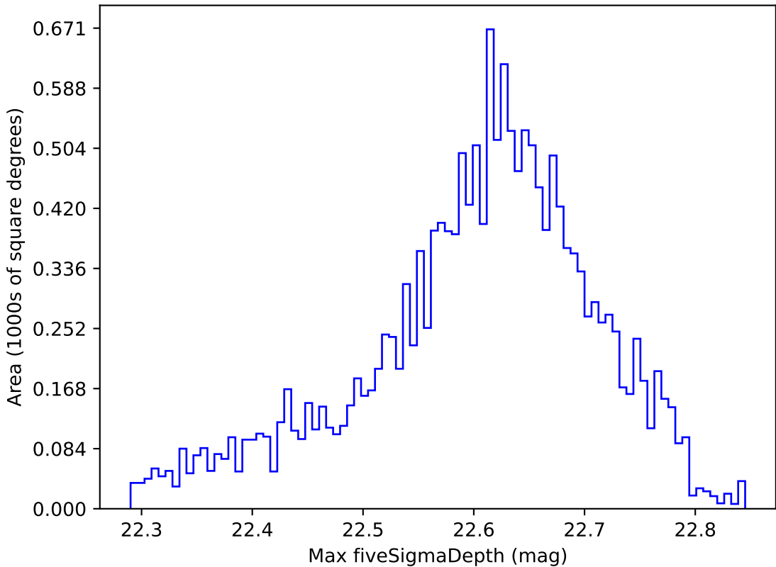
too_elab_r16_d2_griz_v3.4_10yrs WFD y band: Max fiveSigmaDepth
