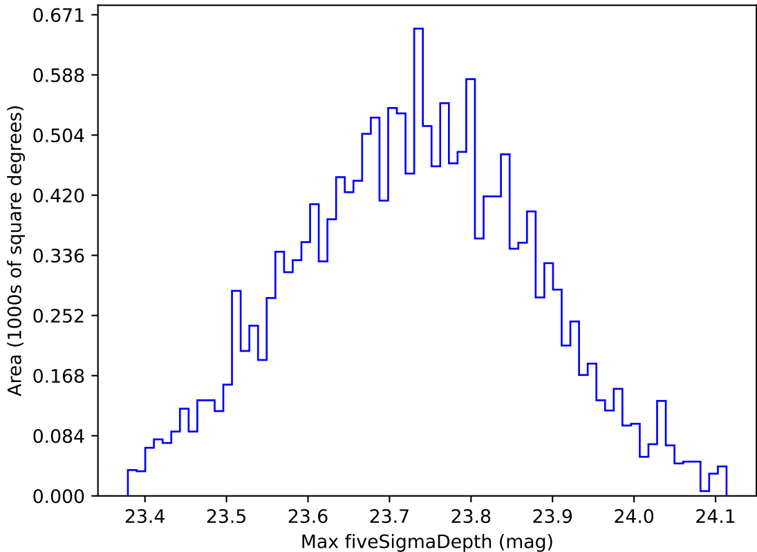
too_elab_r16_d2_griz_v3.4_10yrs WFD u band: Max fiveSigmaDepth
