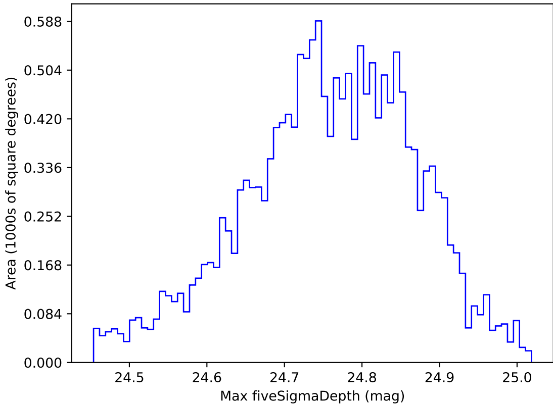
too_elab_r16_d2_griz_v3.4_10yrs WFD r band: Max fiveSigmaDepth
