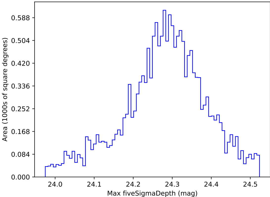
too_elab_r16_d2_griz_v3.4_10yrs WFD i band: Max fiveSigmaDepth
