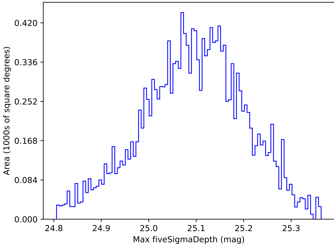
too_elab_r16_d2_griz_v3.4_10yrs WFD g band: Max fiveSigmaDepth
