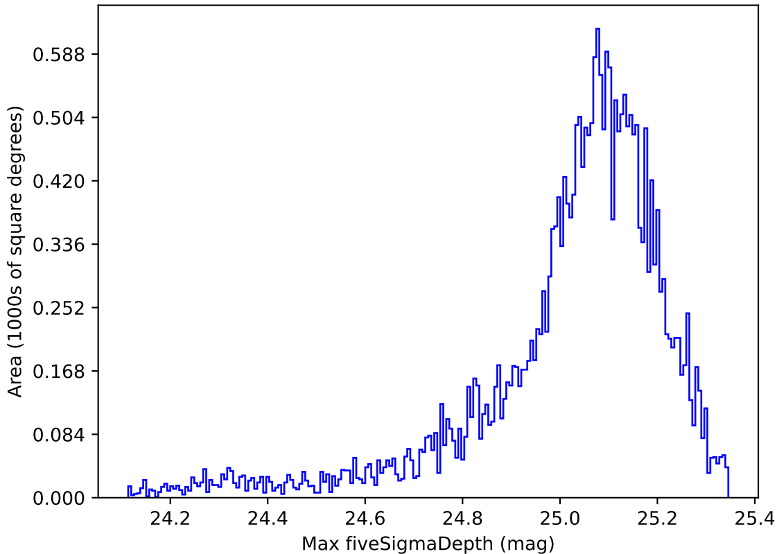
too_elab_r16_d2_griz_v3.4_10yrs All sky g band: Max fiveSigmaDepth
