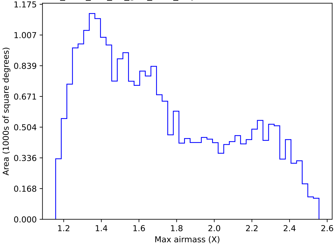
too_elab_r16_d2_griz_v3.4_10yrs Yr 1 r band: Max airmass
