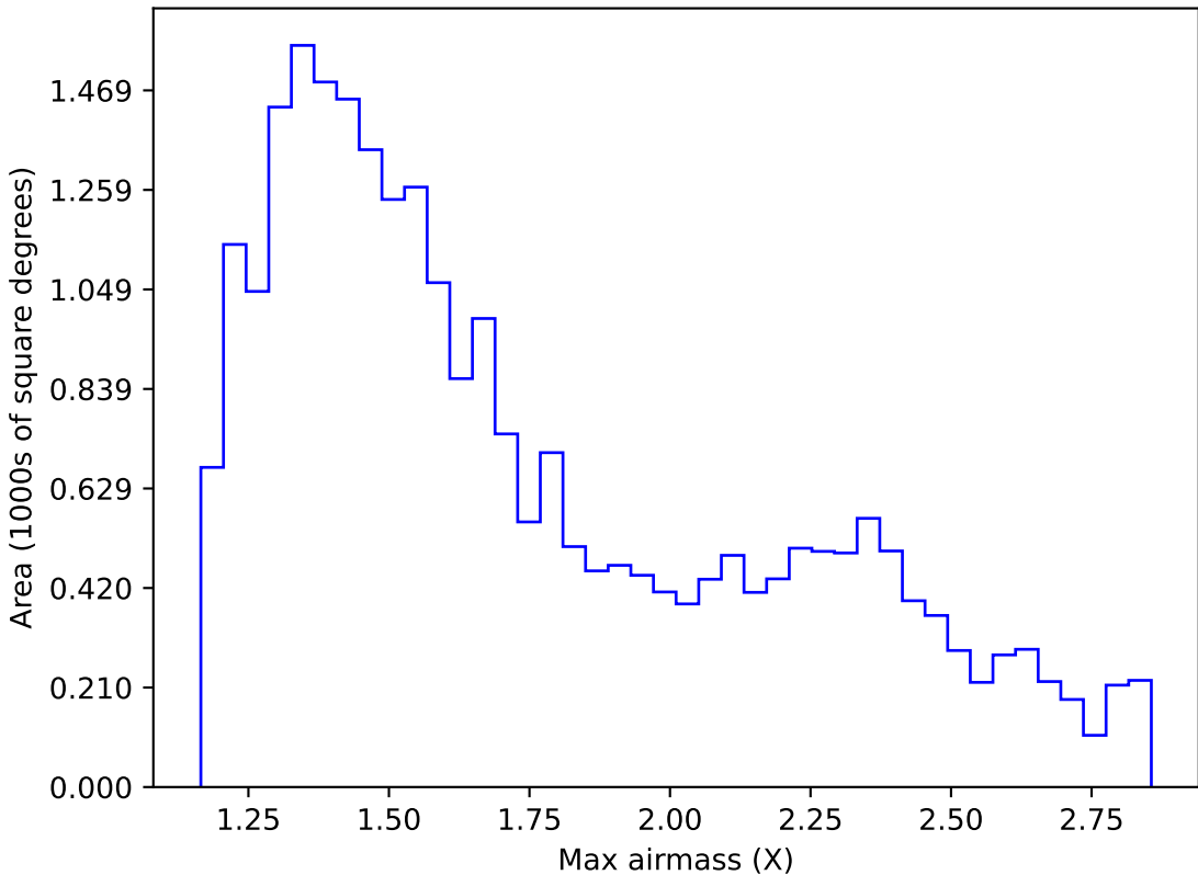
too_elab_r16_d2_griz_v3.4_10yrs Yr 1 i band: Max airmass
