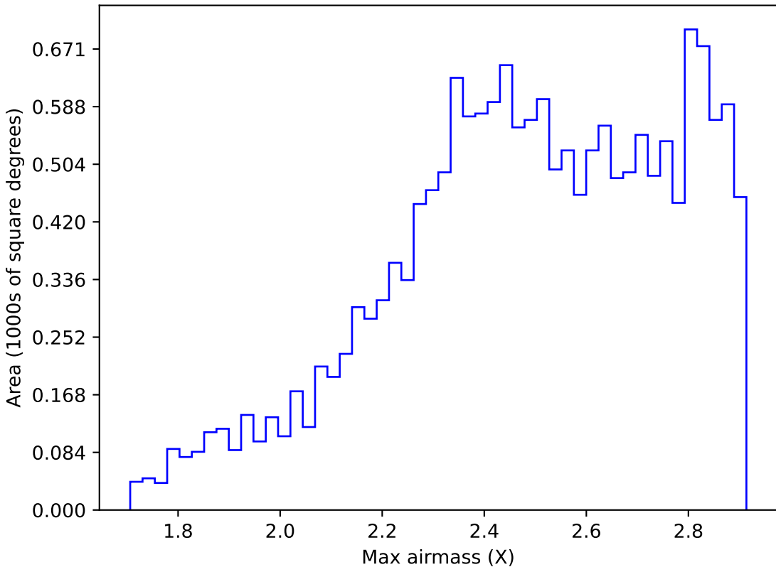
too_elab_r16_d2_griz_v3.4_10yrs WFD z band: Max airmass
