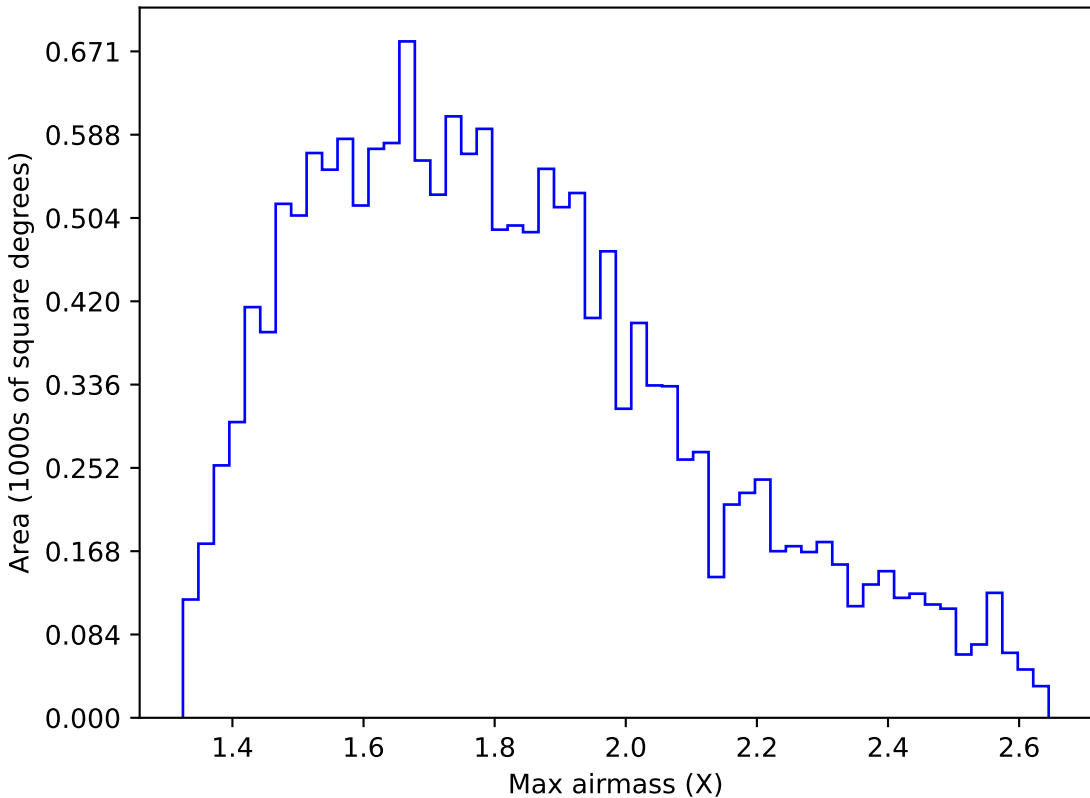
too_elab_r16_d2_griz_v3.4_10yrs WFD u band: Max airmass
