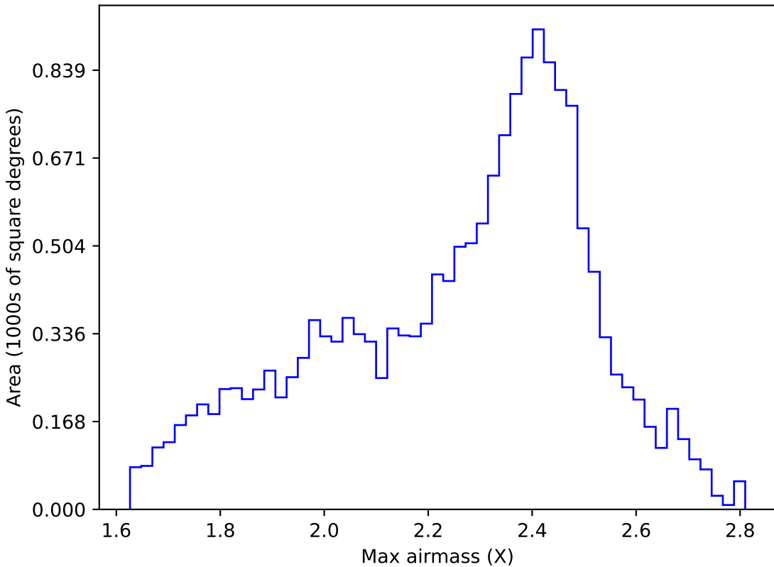
too_elab_r16_d2_griz_v3.4_10yrs WFD r band: Max airmass
