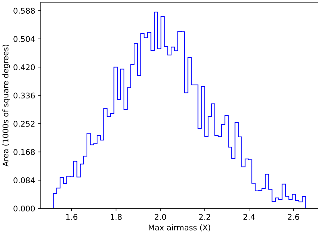
too_elab_r16_d2_griz_v3.4_10yrs WFD g band: Max airmass
