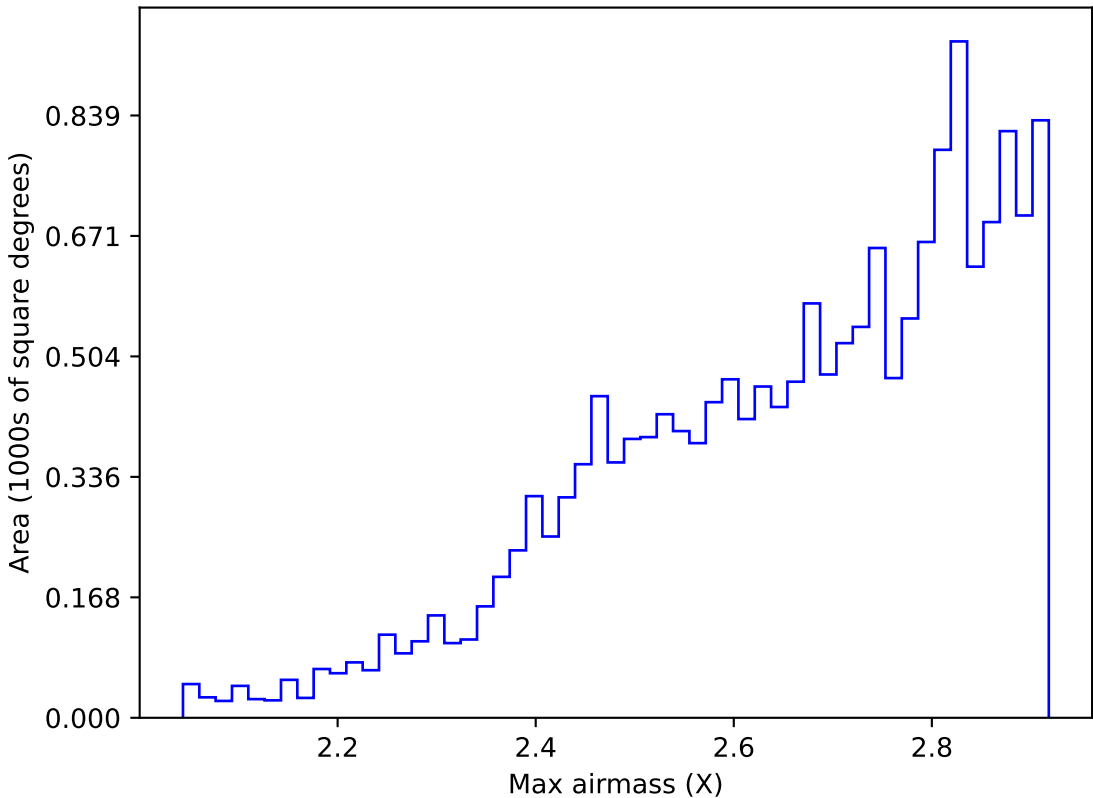
too_elab_r16_d2_griz_v3.4_10yrs WFD all bands: Max airmass
