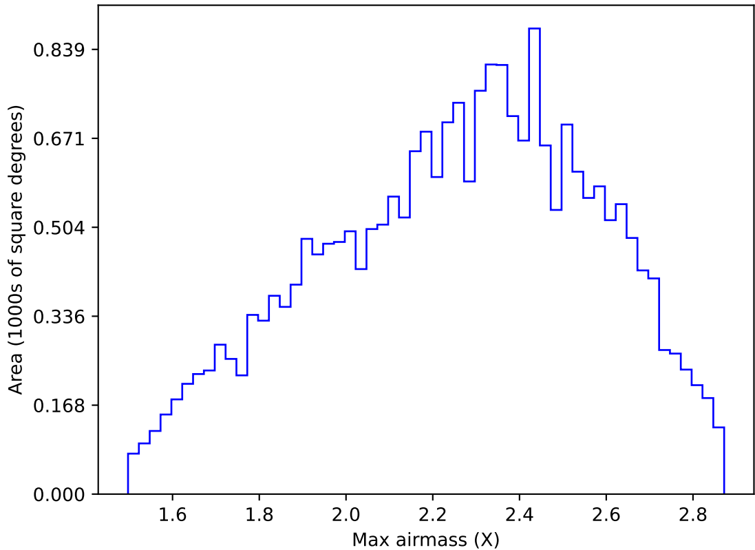
too_elab_r16_d2_griz_v3.4_10yrs All sky y band: Max airmass
