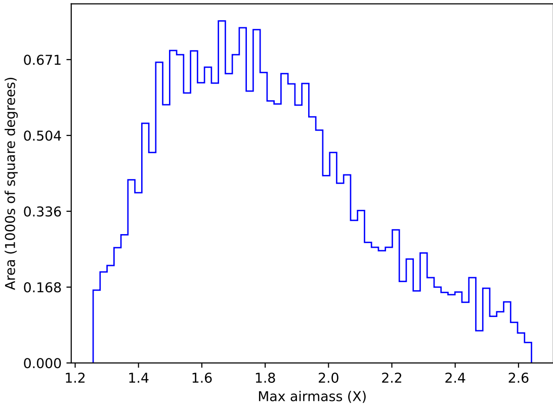
too_elab_r16_d2_griz_v3.4_10yrs All sky u band: Max airmass
